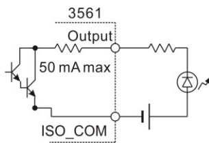
驱动 LED 灯
